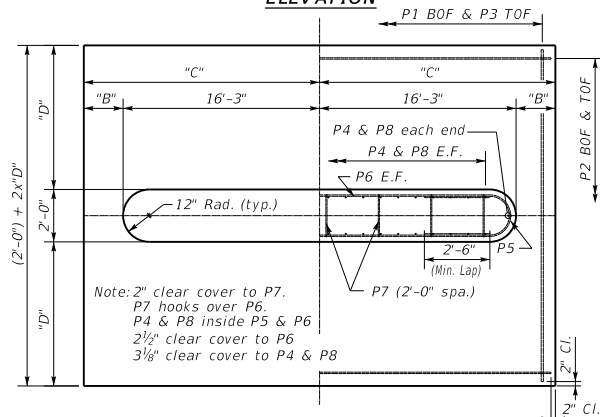
PLAN OF FOOTING
