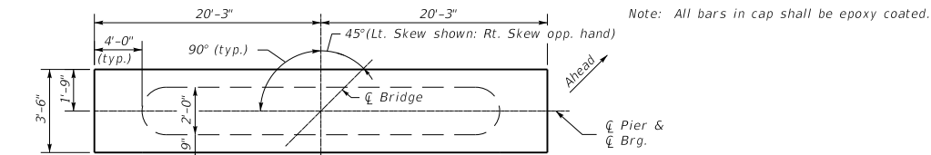
PLAN OF CAP
