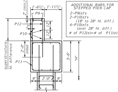
STEPPED CAP (if necessary)
